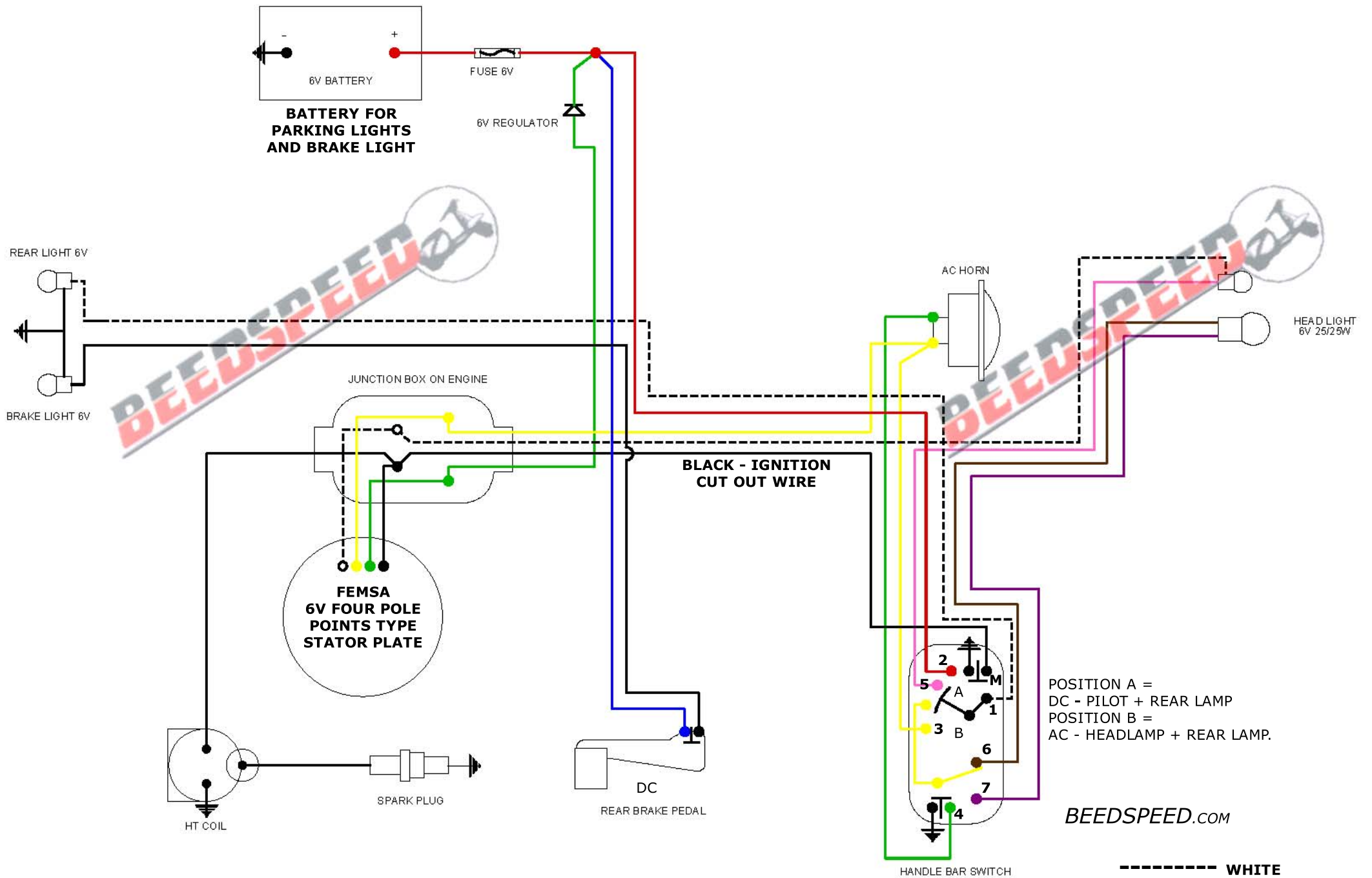
SPANISH MOTOVESPA 150S BATTERY MODEL 1963 -1965
